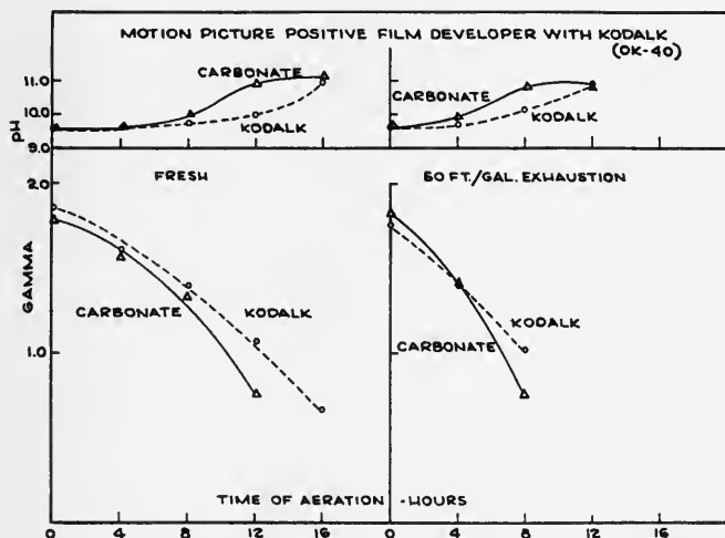
FIG. 6. Showing the difference in behavior between two developers of the same formula, DK-40 compounded with (a) Kodalk and (b) an equivalent quantity of sodium carbonate.
